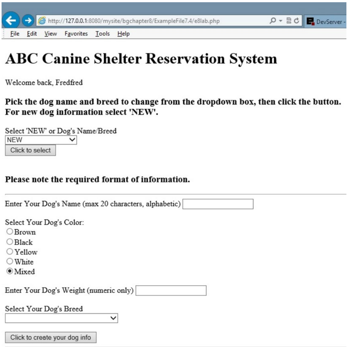
Figure 8-2. The lab.php file with NEW selected
